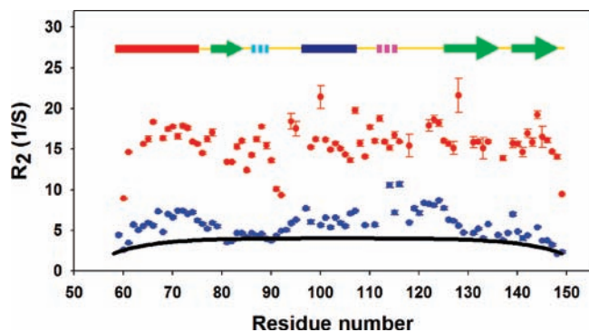
Figure 7. Plots of ^{15}\text{N} R_2 relaxation rates for wild-type CTL9 (red ●) and the cold denatured state of I98A CTL9 (blue ●). The black solid line (—) is the best fit to the phenomenological model of Schwalbe and co-workers. Data were collected at 12 °C for both proteins.
