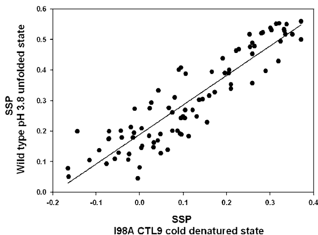
Figure 8. Comparison of the SSP scores determined for the pH 3.8 unfolded state of wild type CTL9 with those determined for the cold denatured state of I98A CTL9. The SSP scores for the pH 3.8 unfolded state were previously reported. 60
