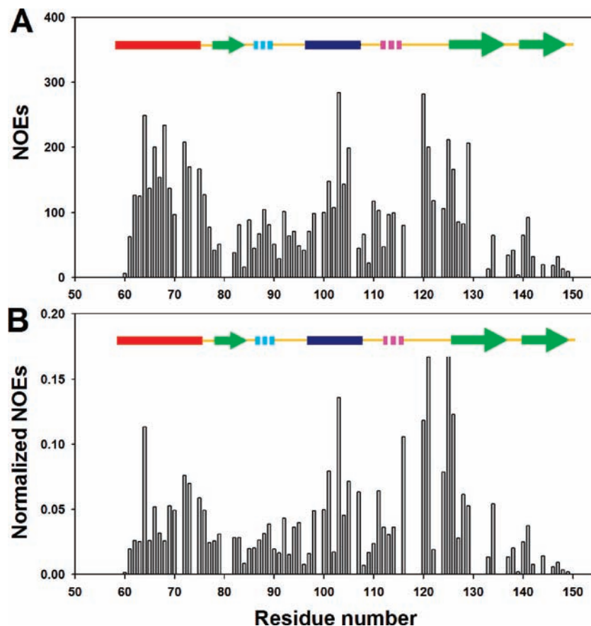
Figure 6. Summary of NOEs observed for I98A CTL9 at pH 5.7, 12 °C. (A) Plot of the volume of the sequential amide proton NOEs versus residue number. (B) Plot of normalized sequential amide proton NOEs versus residue number. Peak volumes are normalized as the ratio of observed d_{NN}(i,i+1) NOE crosspeaks to the diagonal peaks.
