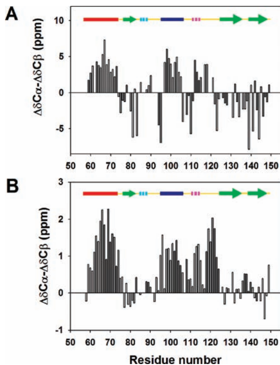
Figure 3. Plots of the difference in the ^{13}\text{C}_\alpha secondary shifts and the ^{13}\text{C}_\beta secondary shifts for (A) The native state of wild-type CTL9, (B) the cold denatured state of I98A CTL9. Note that the scale is different in panel A and panel B. Assignments were obtained at pH 5.7, 12 °C. A schematic diagram of the elements of secondary structure of the native state of CTL9 is shown at the top of each panel, with solid bars, hashed bars, and open arrows indicating \alpha helix, 3–10 helix, and \beta -strand structure, respectively. The color coding corresponds to that used in Figure 1.
