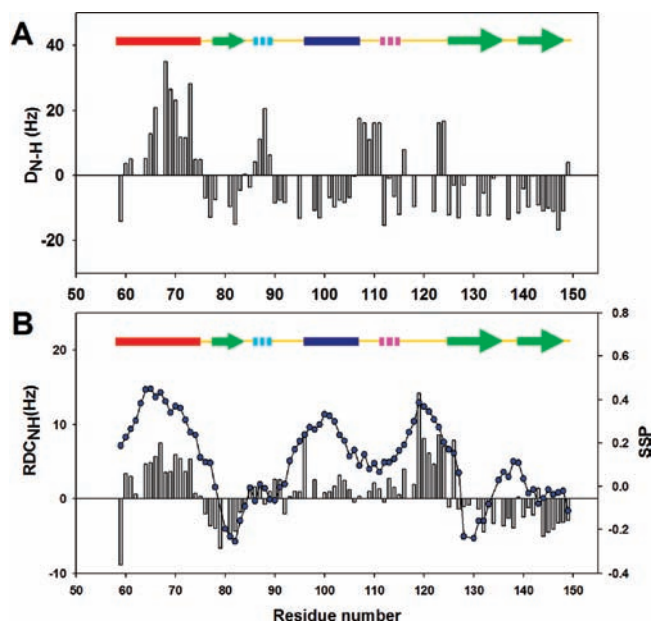
Figure 5. Residual dipolar couplings for CTL9 and the I98A mutant. Measurements were made at pH 5.7, 12 °C. (A) Plot of D_{\text{NH}} for the wild-type CTL9 versus residue number. (B) Plot of D_{\text{NH}} (black bars) and SSP scores (●) for I98A CTL9 versus residue number. A schematic diagram of the elements of secondary structure of the native state of CTL9 is shown at the top of each panel.
