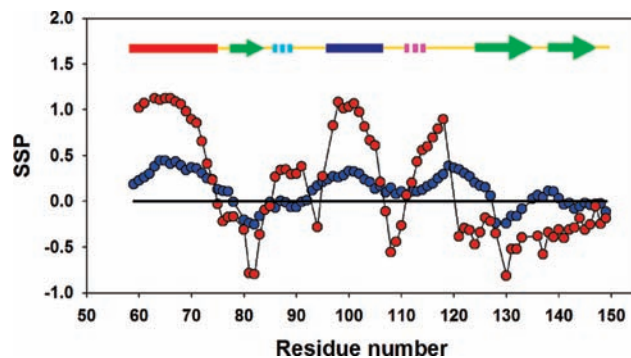
Figure 4. SSP analysis of wild-type CTL9 (red ●) and I98A CTL9 (blue ●) at pH 5.7, 12 °C. A schematic diagram of the elements of secondary structure of the native state of CTL9 is shown at the top of the figure.
